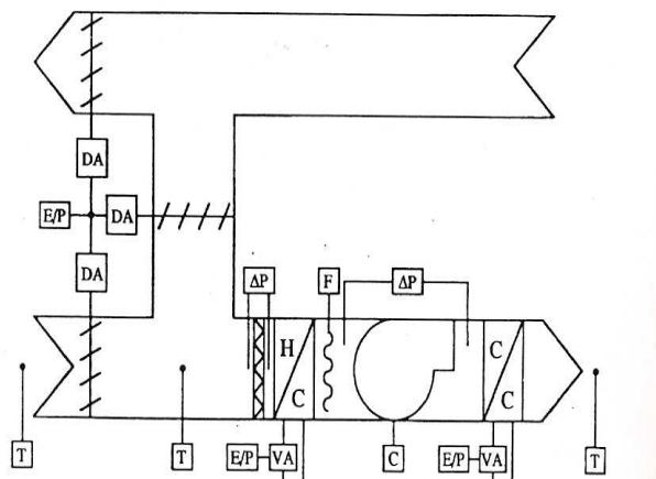
Fig. 3. System Diagram for the Air Handler
